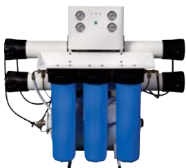
RO water filter The PureFlo RO water filter removes 95% of minerals from supply water to reduce scale build-up and maintenance
